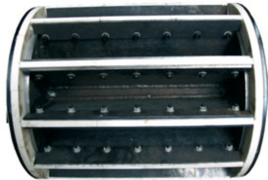
Installed rotor cell with ceramic wear elements
