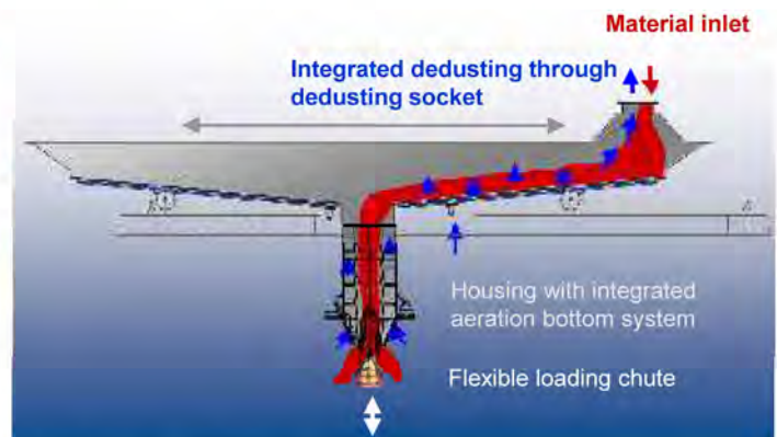
Loading and dedusting prinzipl
